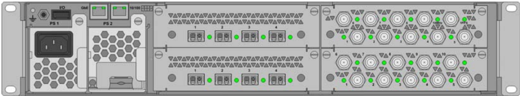
Figure 2. Digital Content Manager (DCM) Model D9900 Rear Panel with AC and DC power supplies, 2 GbE cards, 1 ASI card and 1 ASI SFN card.
